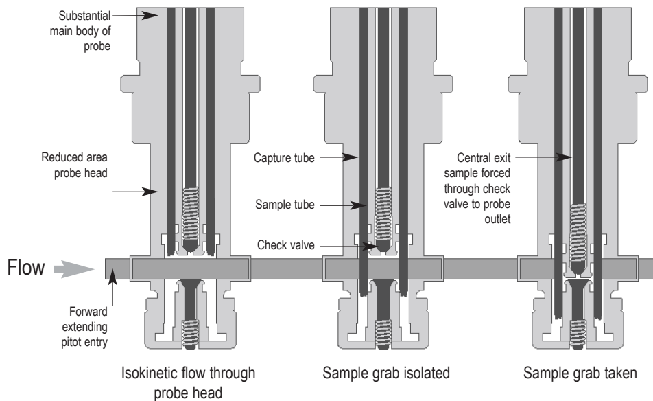
Three stage positive displacement action
